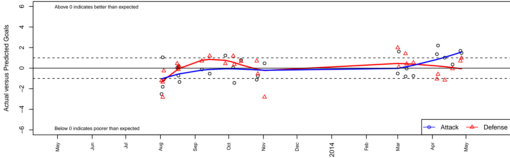
FC Columbia County G99 Dots are actual minus expected GF (blue circles) and GA (red triangles). Blue line is smoothed change in attack strength. Red is smoothed change in defense strength.
